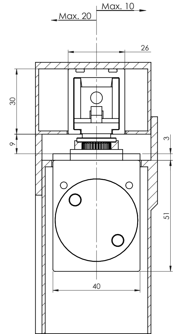
SECTION P-P
