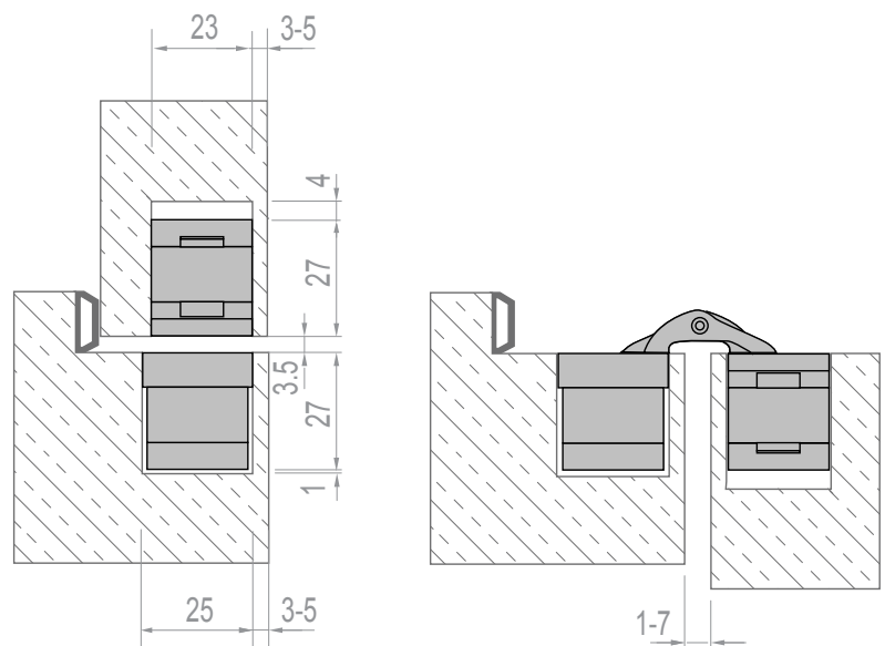
Section of Wood Frame-Door Installation
