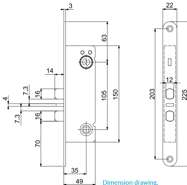
Dimension drawing, Connect 621-35
